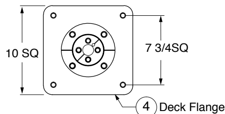
ROOF MOUNT ASSEMBLY
